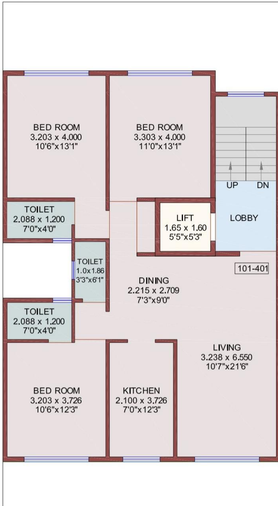
1ST - 4TH FLOOR PLAN
